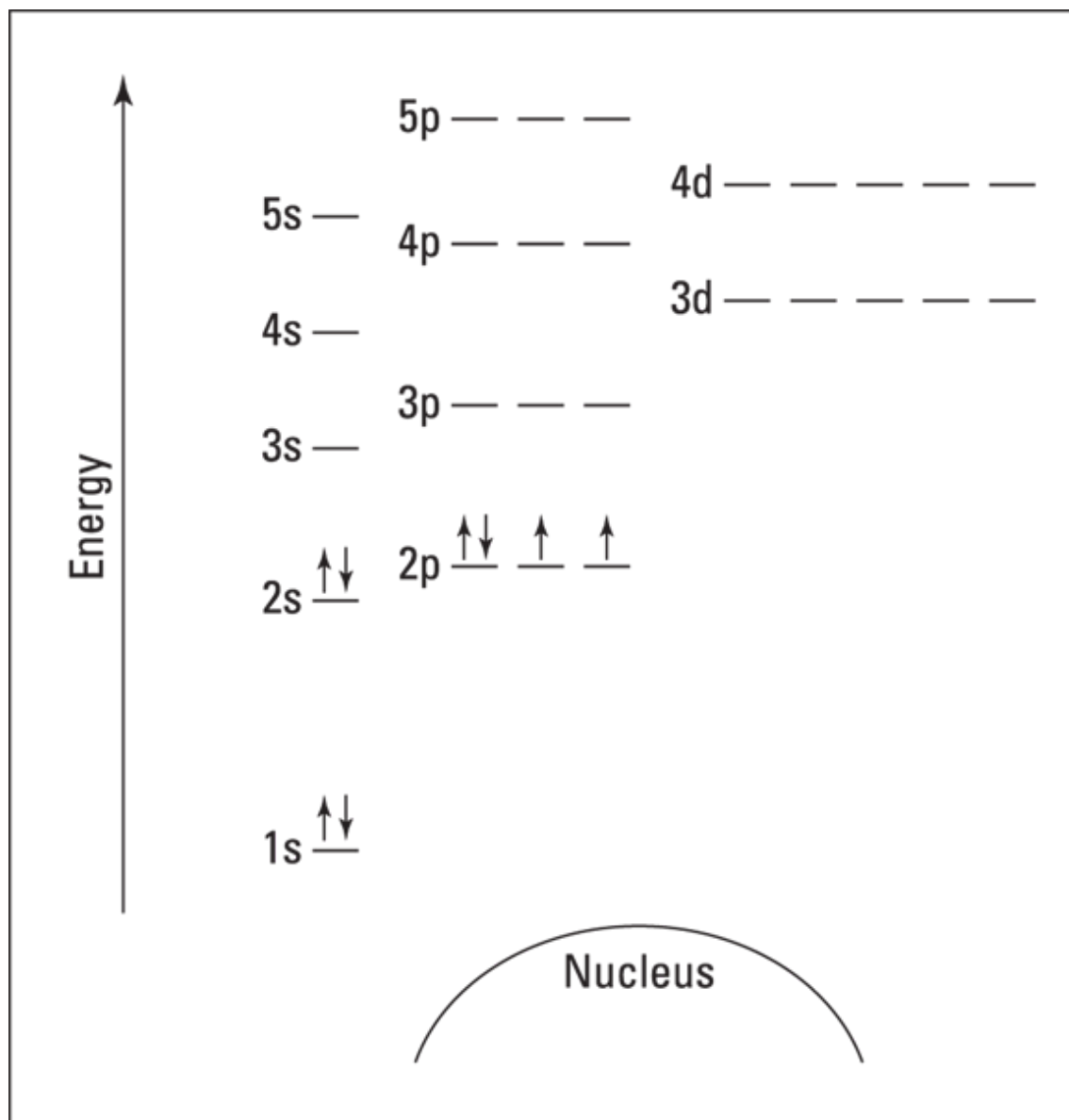
FIGURE 4-7: Energy-level diagram for oxygen.
