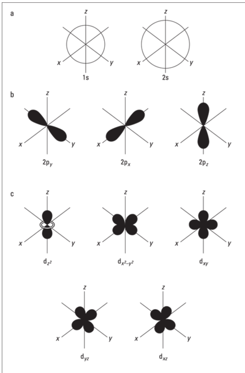
FIGURE 4-4: Shapes of the s (a), p (b), and d (c) orbitals.
