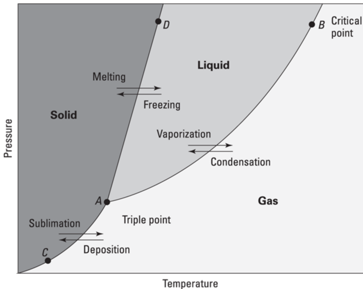
FIGURE 17-1: A general phase diagram.
