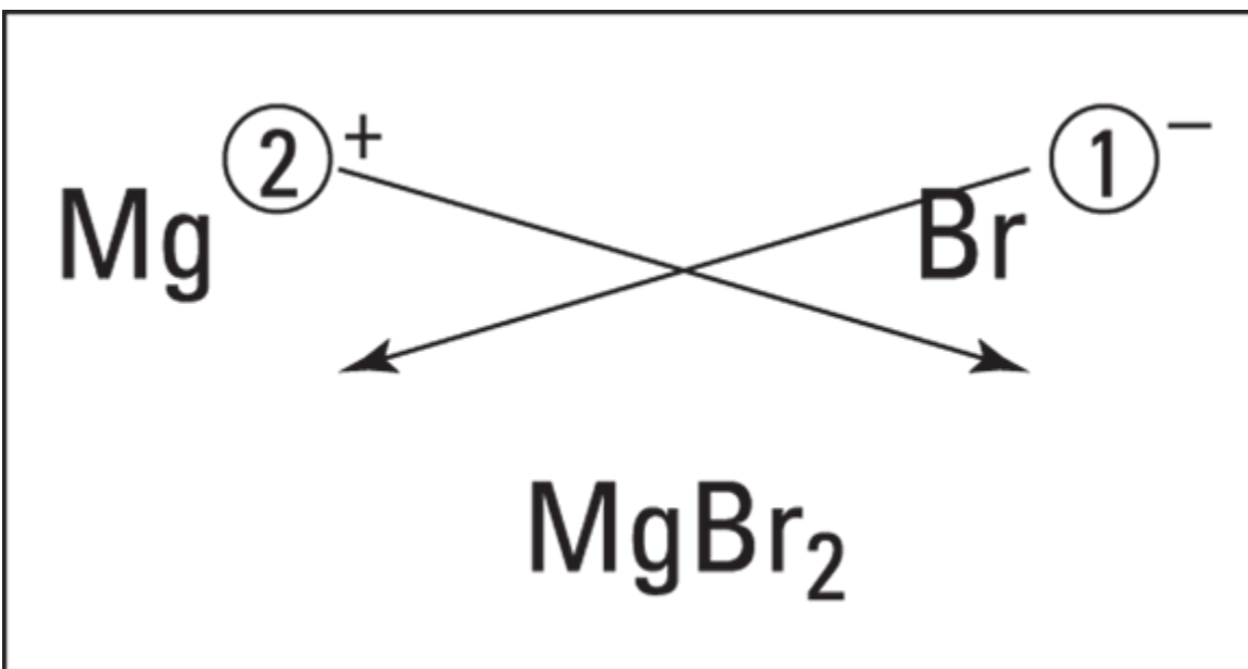
FIGURE 13-3: Figuring the formula of magnesium bromide.
