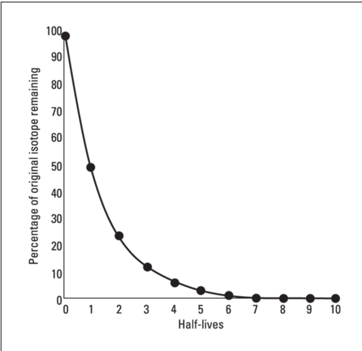
FIGURE 20-2: Decay of a radioactive isotope.
