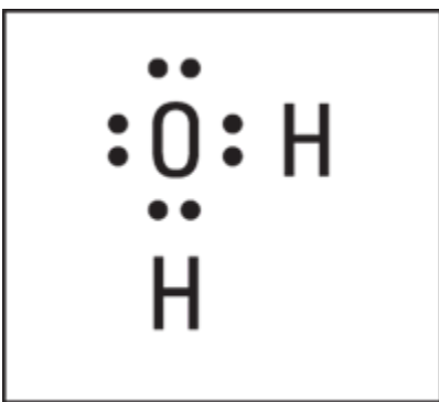
FIGURE 14-6: Electron-dot formula of \text{H}_2\text{O} .
