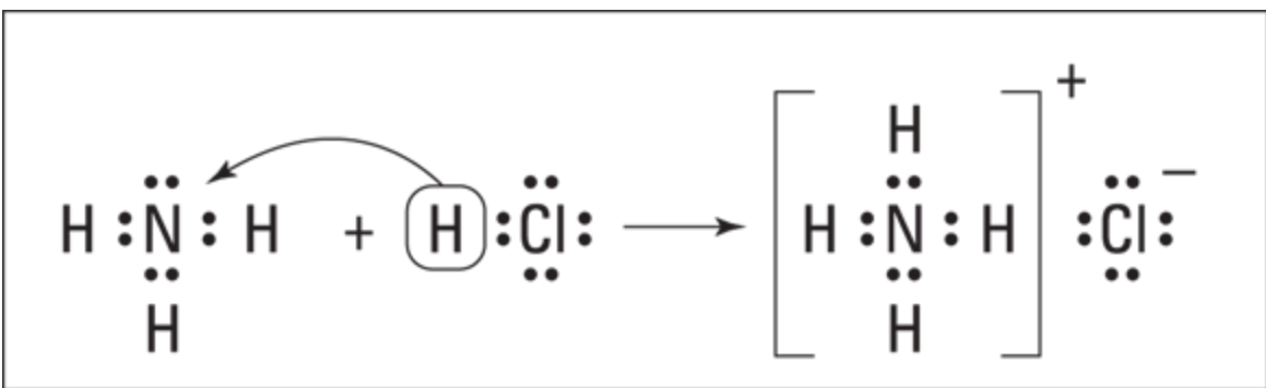
FIGURE 11-1: Reaction of \text{NH}_3 with HCl.
