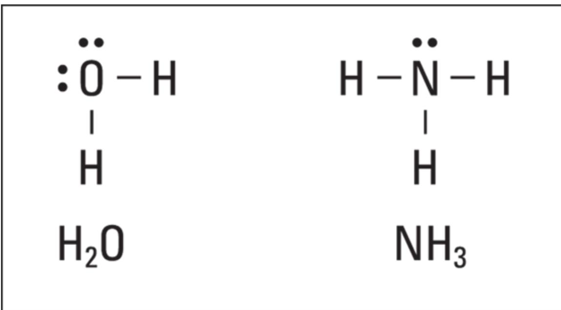
FIGURE 15-5: Lewis formulas for \text{H}_2\text{O} and \text{NH}_3 .
