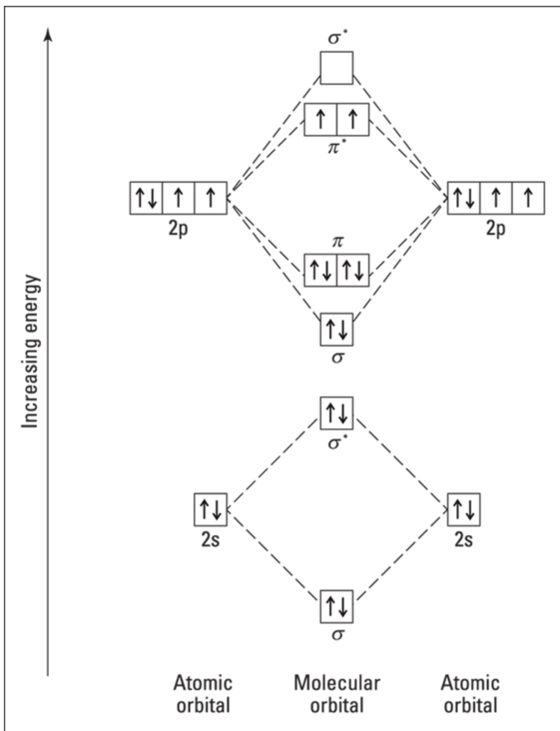
FIGURE 15-11: MO diagram for O_2 (valence-shell electrons only).
