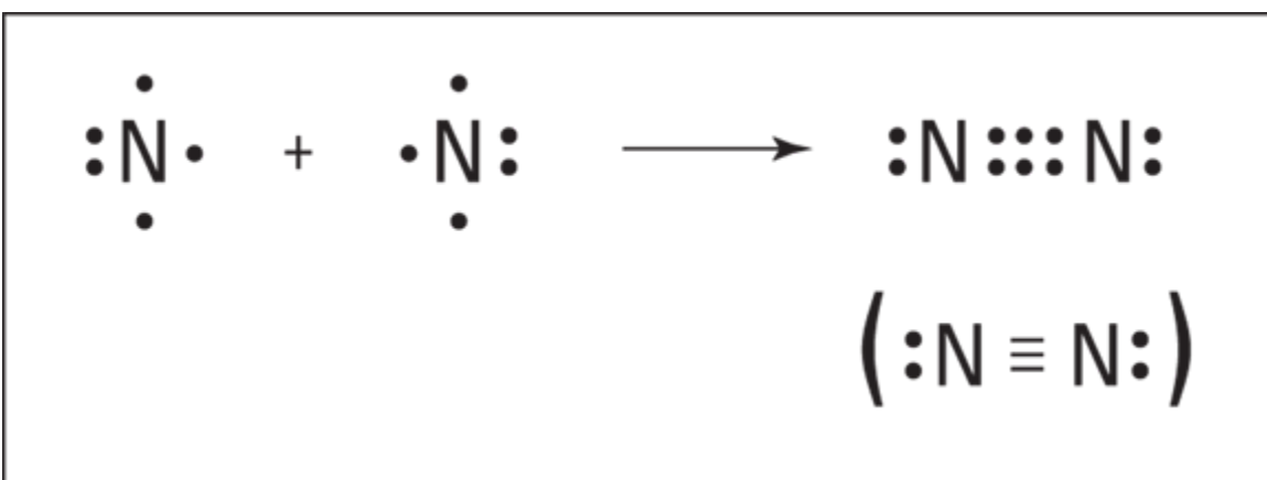
FIGURE 14-3: Triple bond formation in \text{N}_2 .
