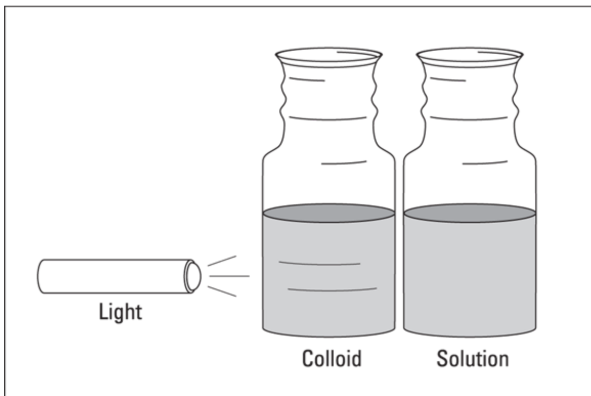
FIGURE 9-5: The Tyndall effect.
