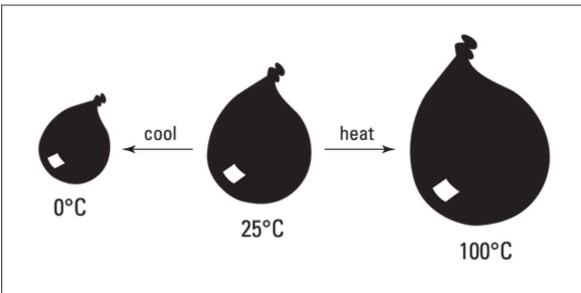
FIGURE 6-4: The temperature-volume relationship of gases — Charles's law.
