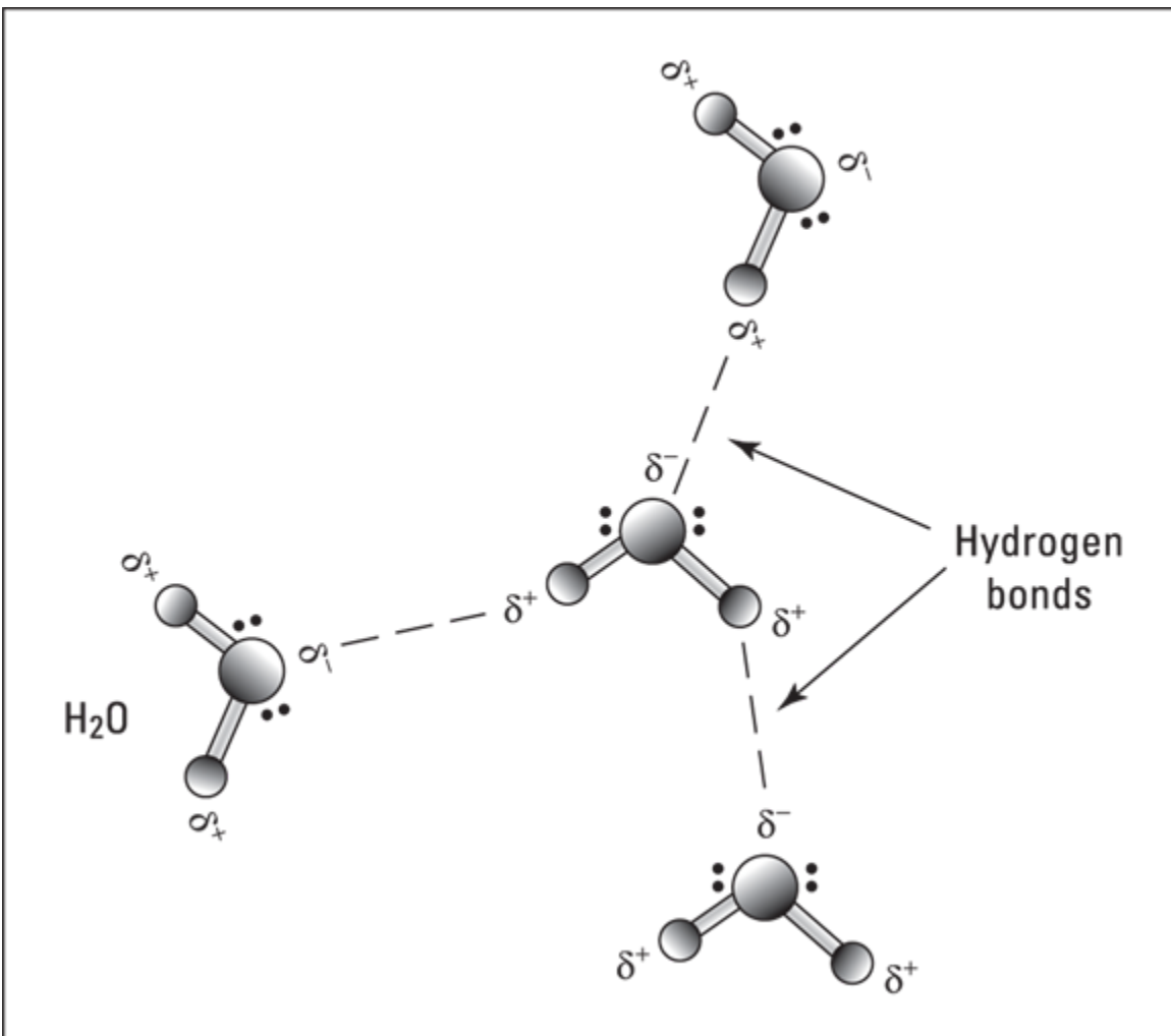
FIGURE 19-2: Hydrogen bonding in water.
