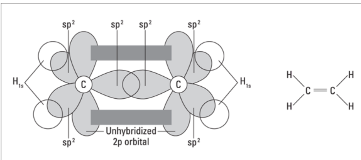
FIGURE 15-7: Hybridization in ethylene.
