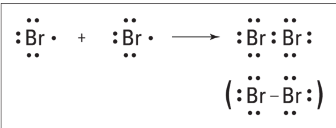
FIGURE 14-2: The covalent bond formation of Br_2 .
