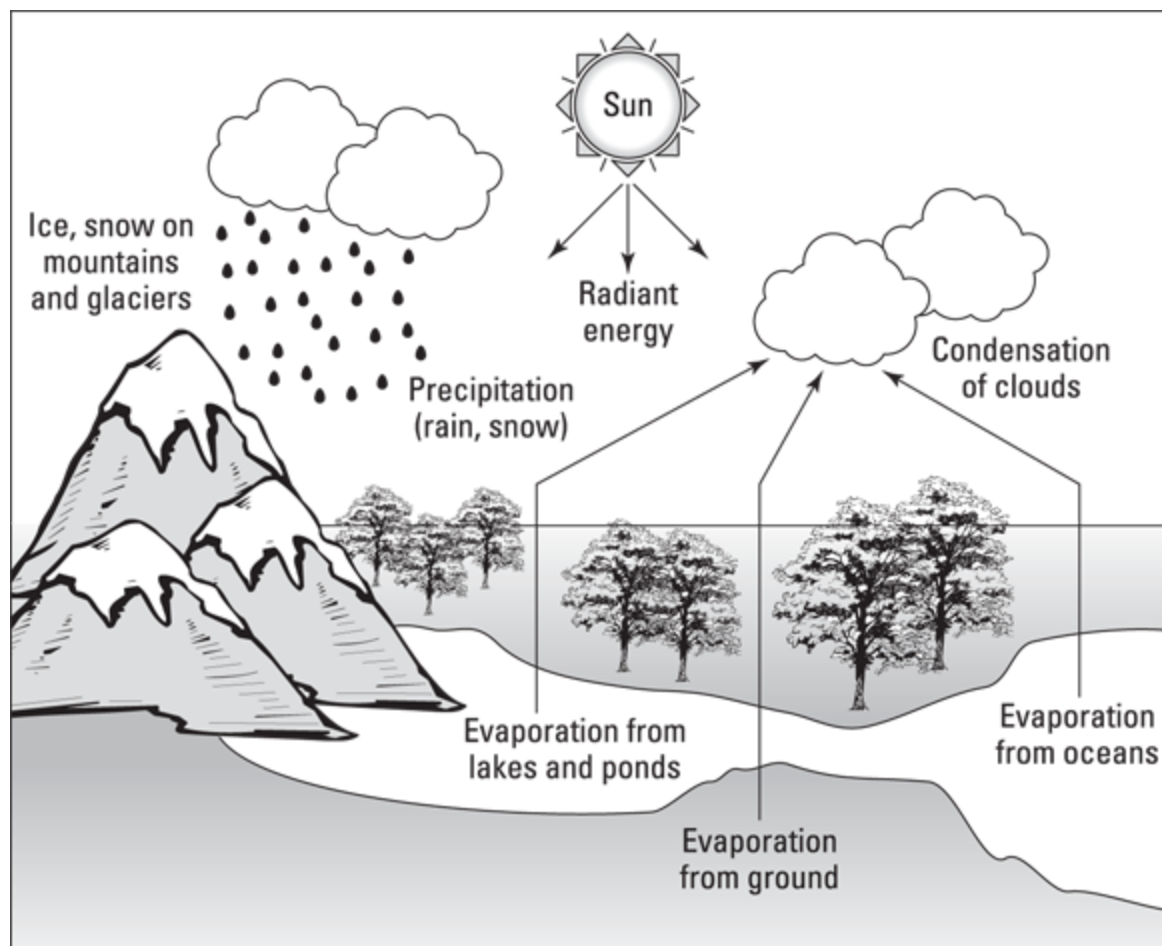
FIGURE 19-1: The water (hydrologic) cycle.
