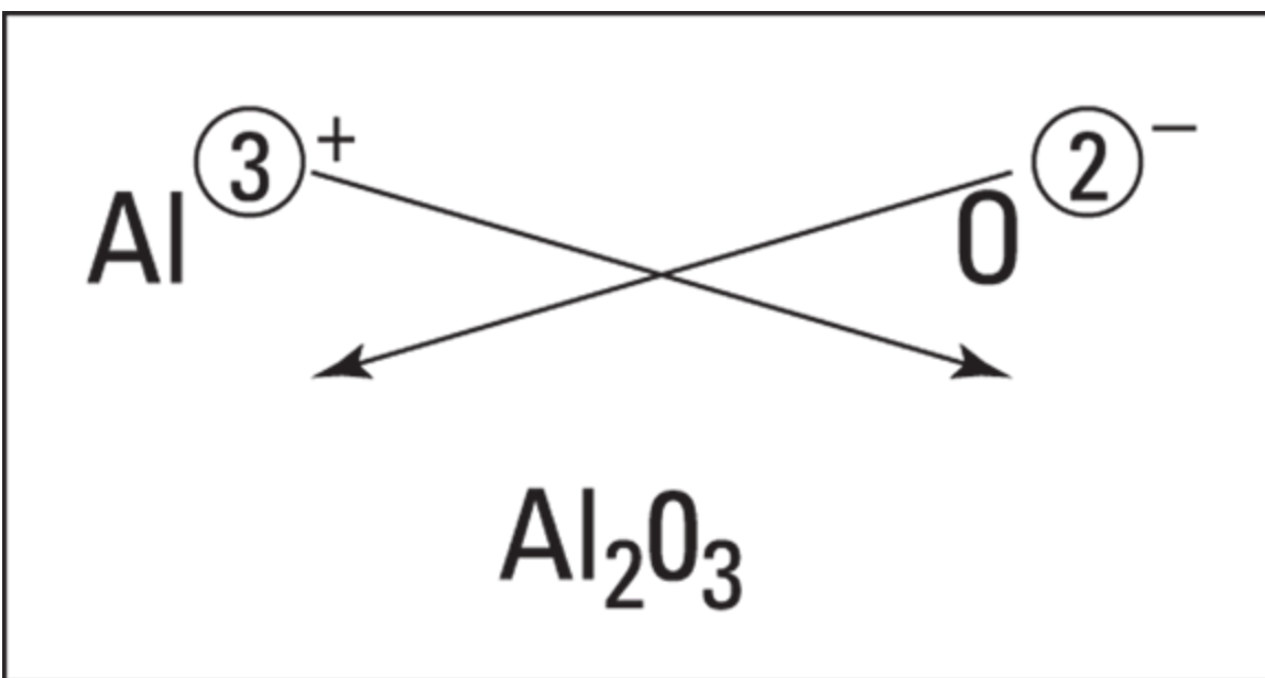
FIGURE 13-4: Figuring the formula of aluminum oxide.
