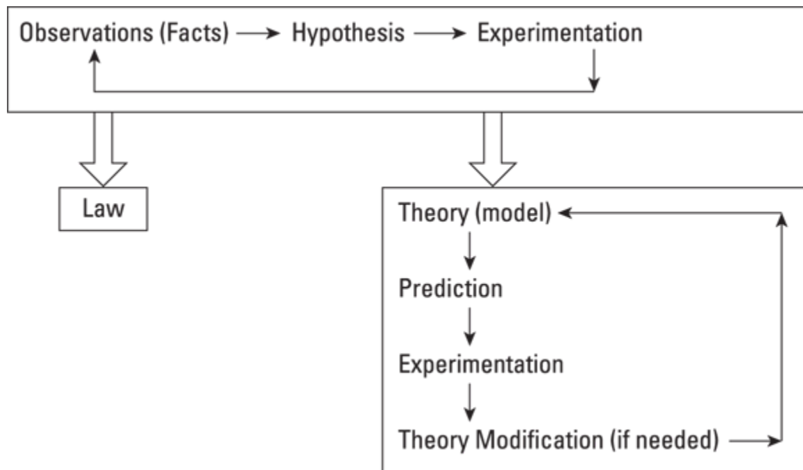
FIGURE 1-1: The scientific method.
