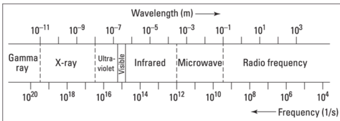
FIGURE 12-2: The electromagnetic spectrum.
