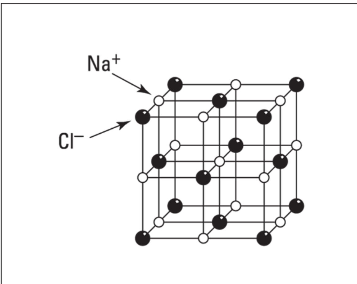
FIGURE 13-2: Crystal structure of sodium chloride.
