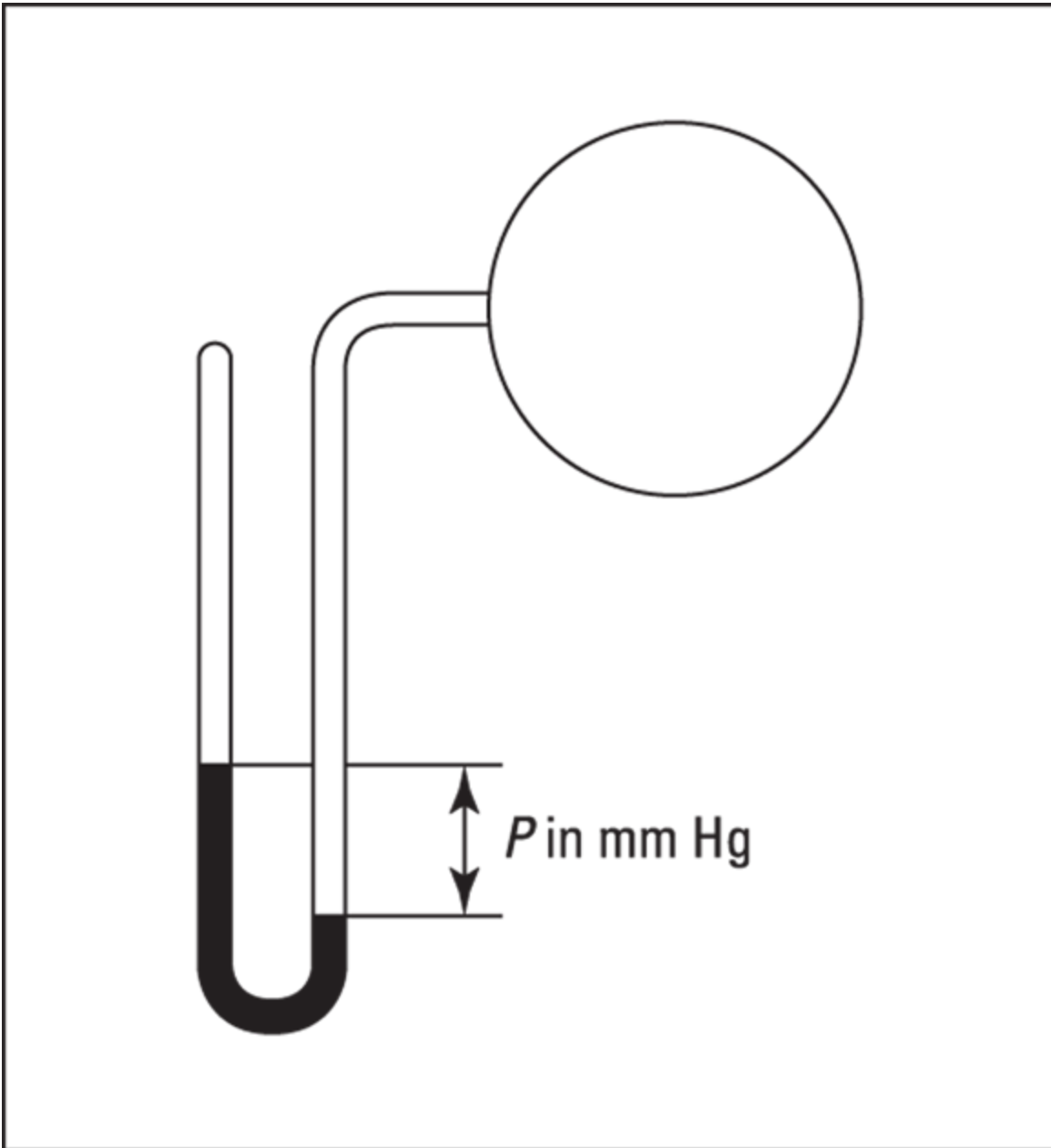
FIGURE 6-2: The manometer.
