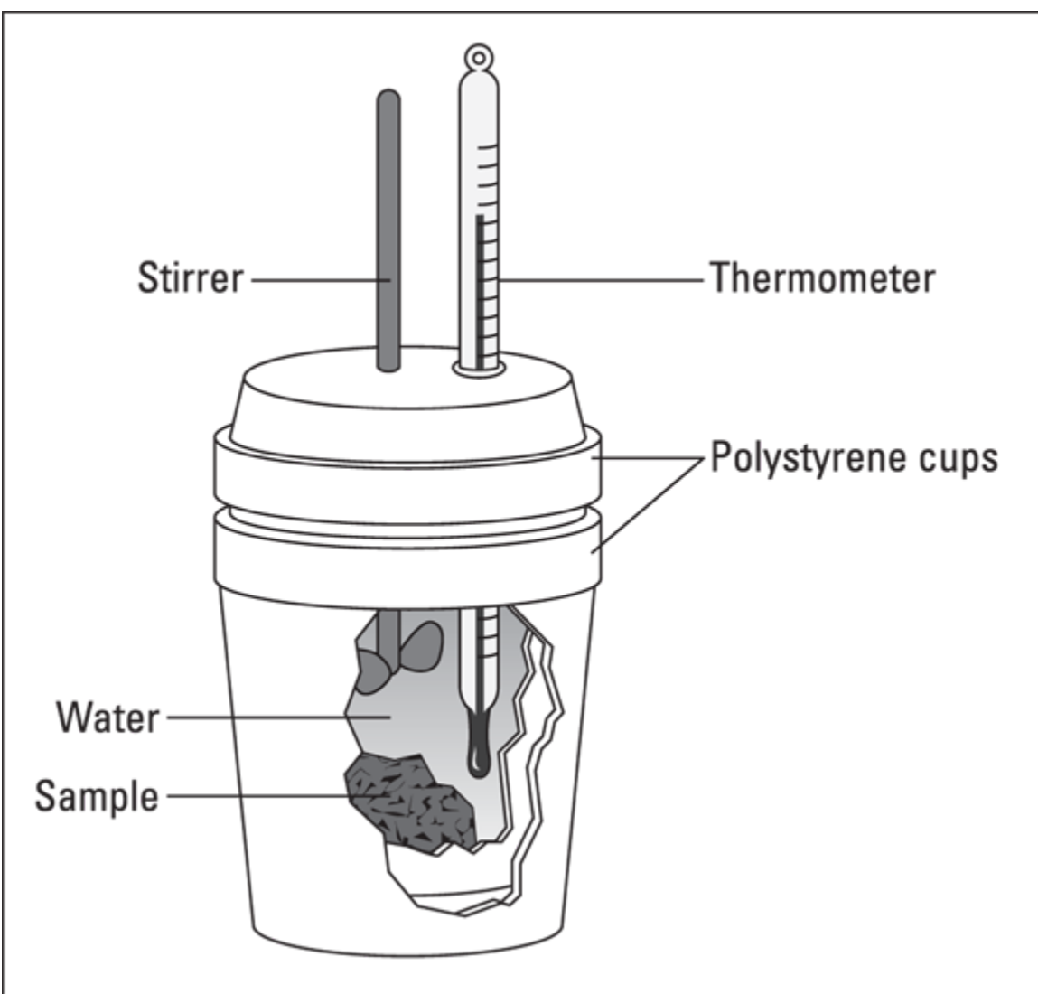
FIGURE 10-1: A constant-pressure (coffee cup) calorimeter.
