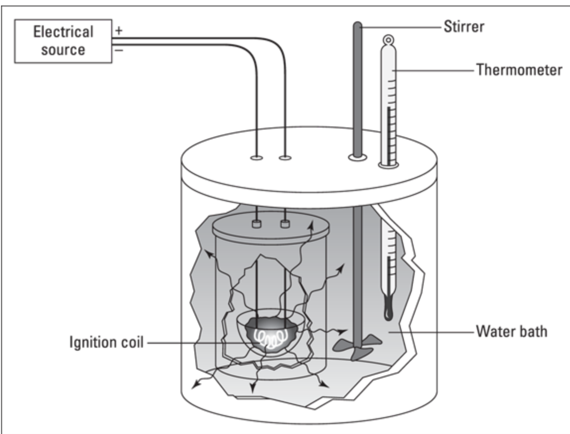
FIGURE 10-2: A constant-volume (bomb) calorimeter.
