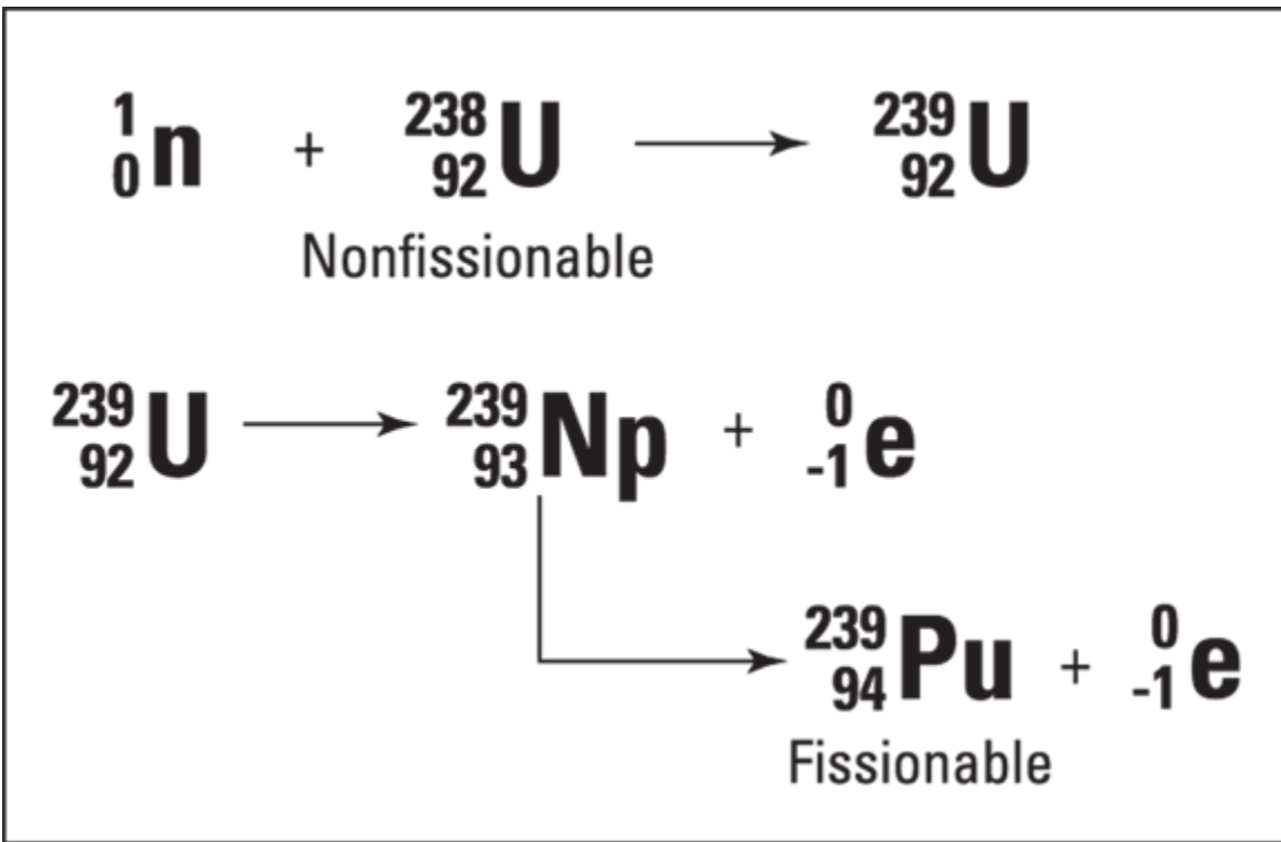
FIGURE 20-4: The breeder reactor process.
