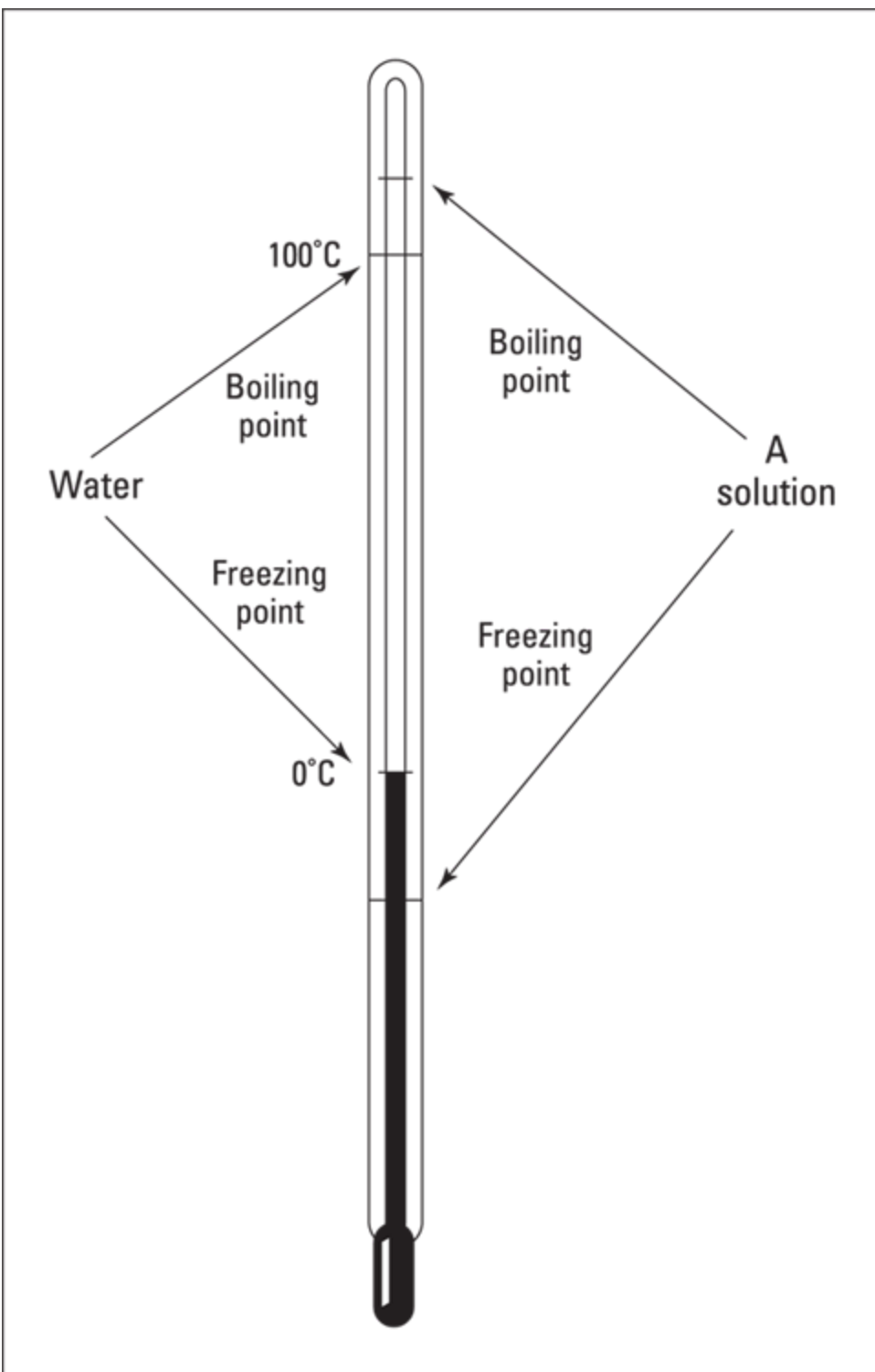
FIGURE 9-2: Boiling-point elevation and freezing point depression of a solution.
