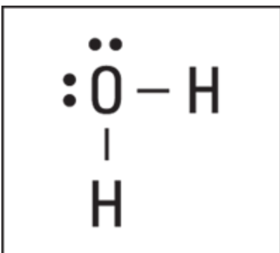
FIGURE 14-7: The Lewis formula for \text{H}_2\text{O} .
