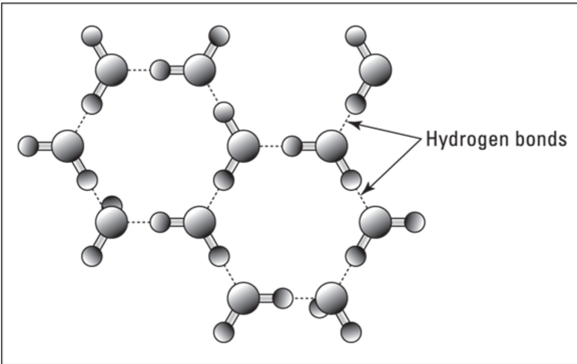
FIGURE 19-3: The structure of ice.
