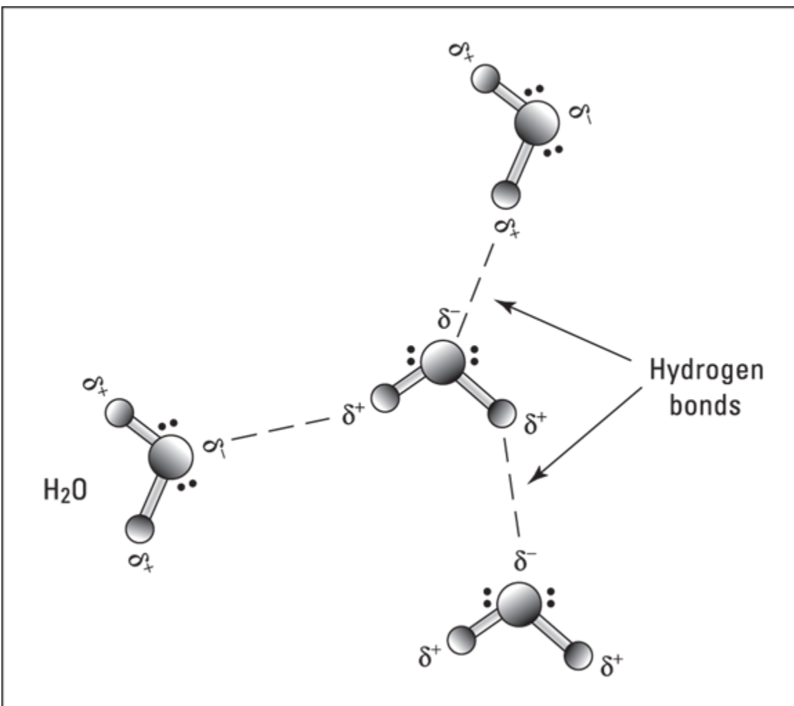
FIGURE 14-14: Hydrogen bonding in water.
