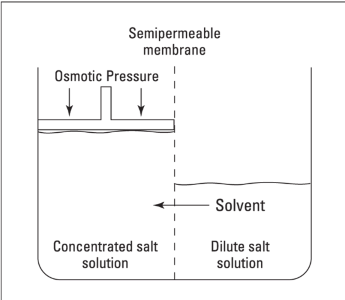
FIGURE 9-3: Osmotic pressure.
