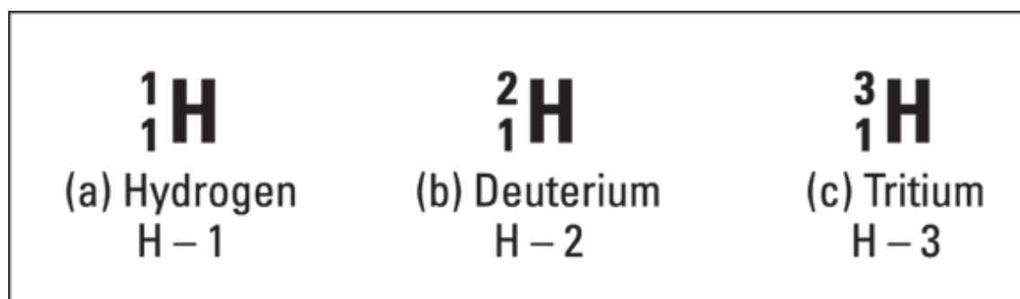
FIGURE 4-8: Hydrogen isotopes containing no neutrons (a), one neutron (b), and two neutrons (c).
