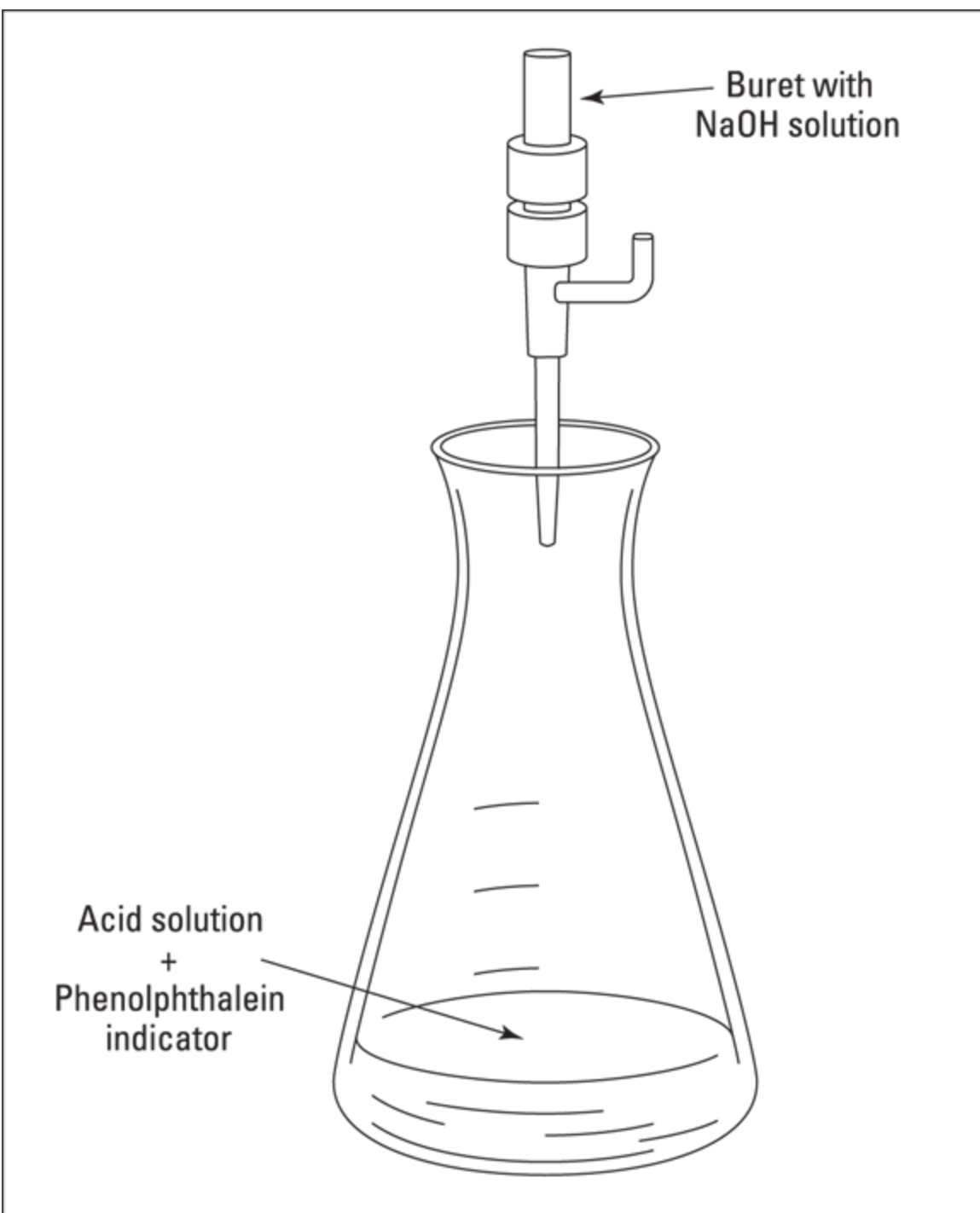
FIGURE 11-2: Titration of an acid with a base.
