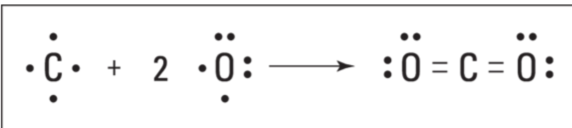
FIGURE 14-4: Formation of carbon dioxide.
