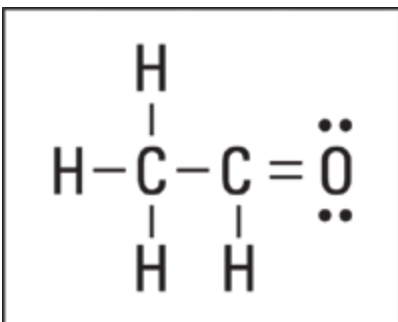
FIGURE 14-9: The Lewis formula for \text{C}_2\text{H}_4\text{O} .
