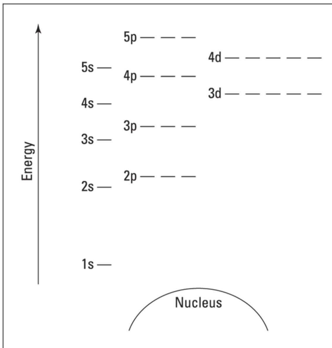
FIGURE 4-5: Energy-level diagram.
