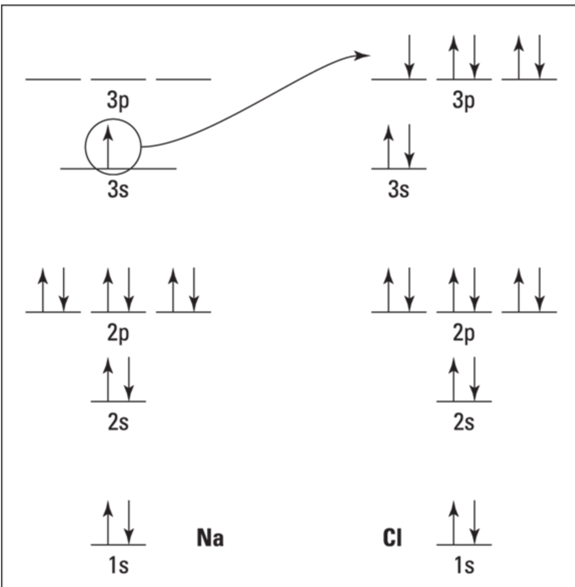
FIGURE 13-1: Energy-level diagrams for sodium and chlorine.
