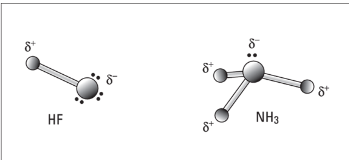
FIGURE 14-12: Polar covalent bonding in HF and NH 3 .
