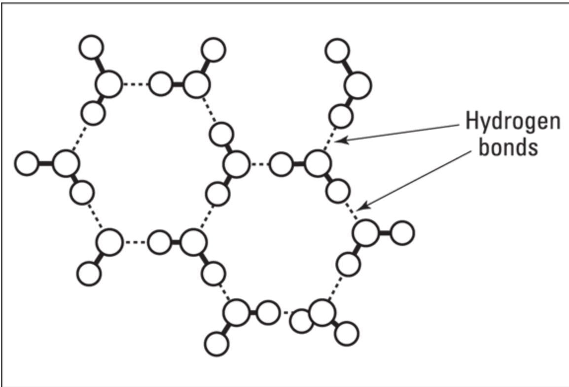
FIGURE 14-15: The structure of ice.
