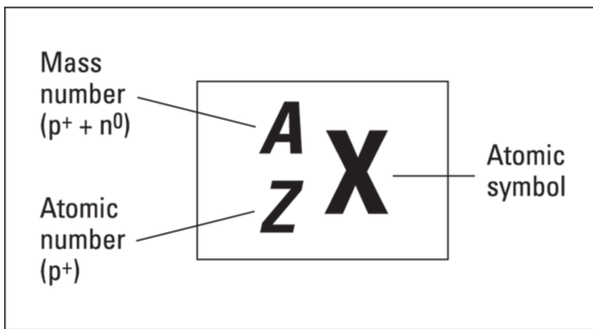
FIGURE 20-1: Representing a specific isotope.
