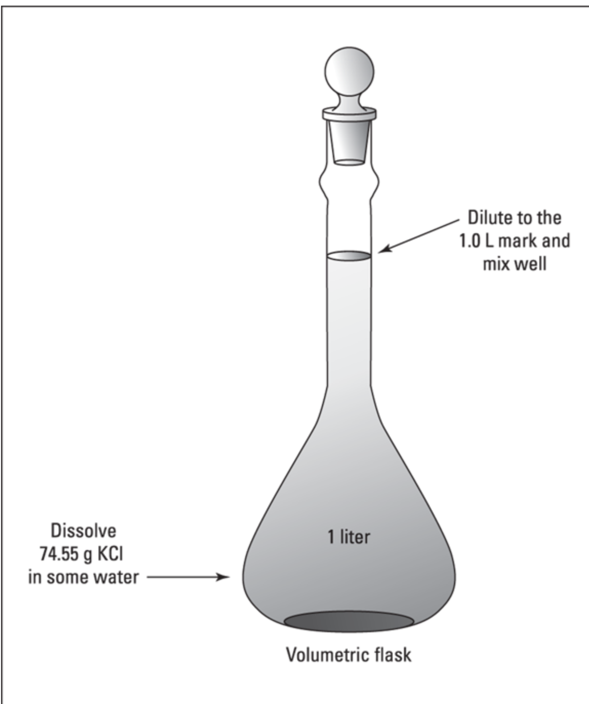
FIGURE 9-1: Making a 1-molar KCl solution.
