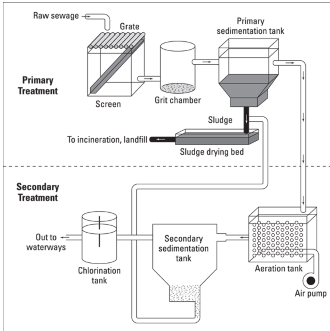
FIGURE 19-5: Primary and secondary sewage treatment.
