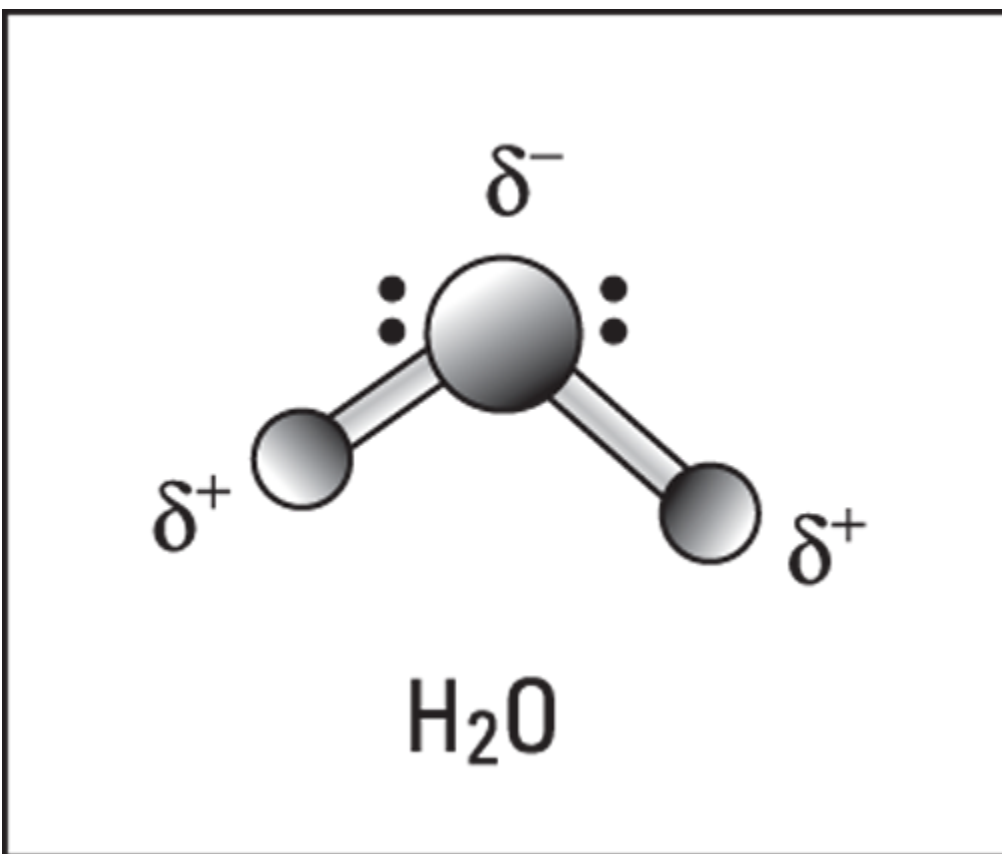
FIGURE 14-13: Polar covalent bonding in water.
