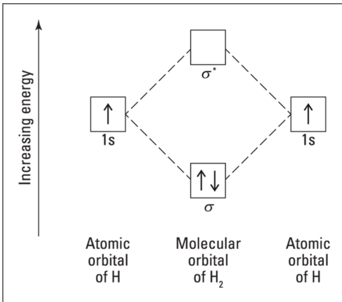
FIGURE 15-10: Molecular orbital diagram for H 2 .
