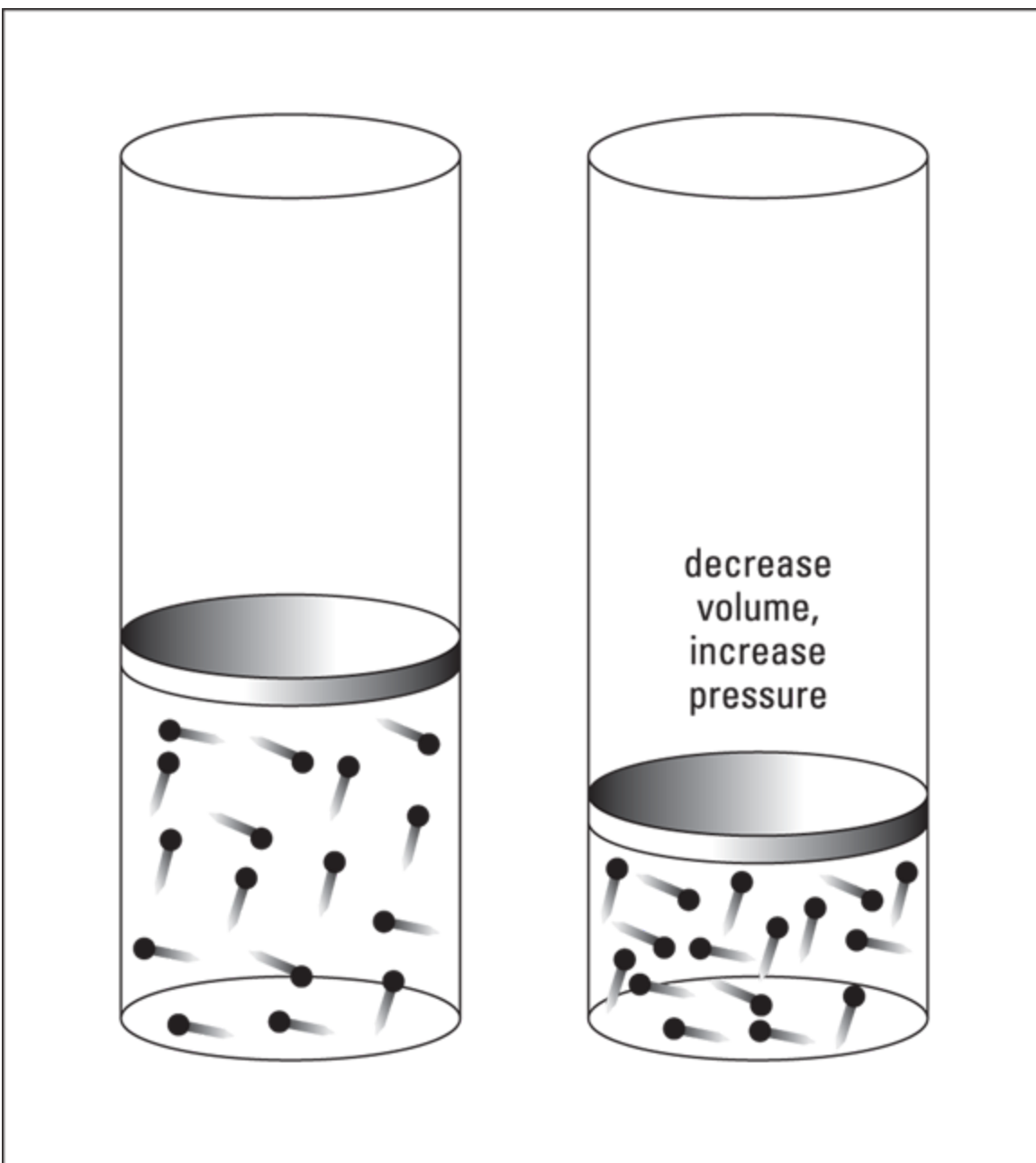
FIGURE 6-3: Pressure-volume relationship of gases — Boyle's law.
