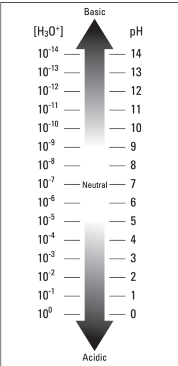
FIGURE 11-3: The pH scale.
