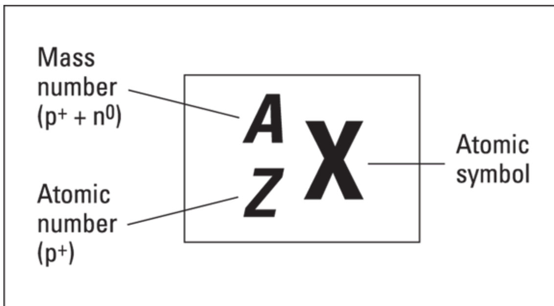
FIGURE 4-1: Representing a specific element.
