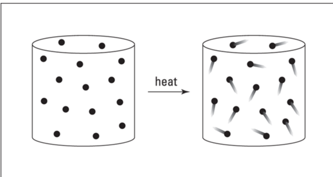
FIGURE 6-5: The pressure-temperature relationship of gases — Gay-Lussac's law.
