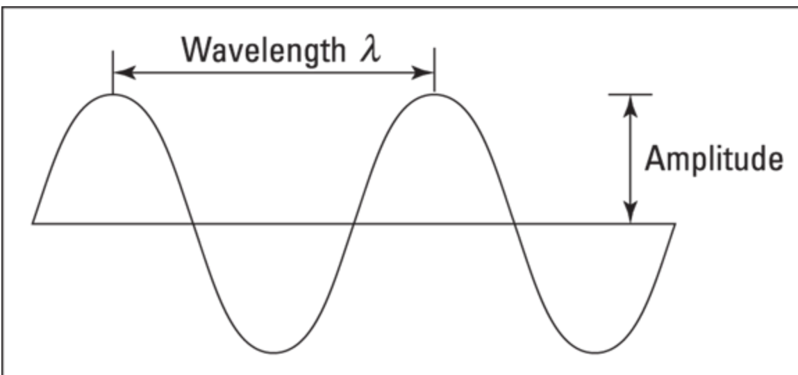
FIGURE 12-1: Properties of waves.
