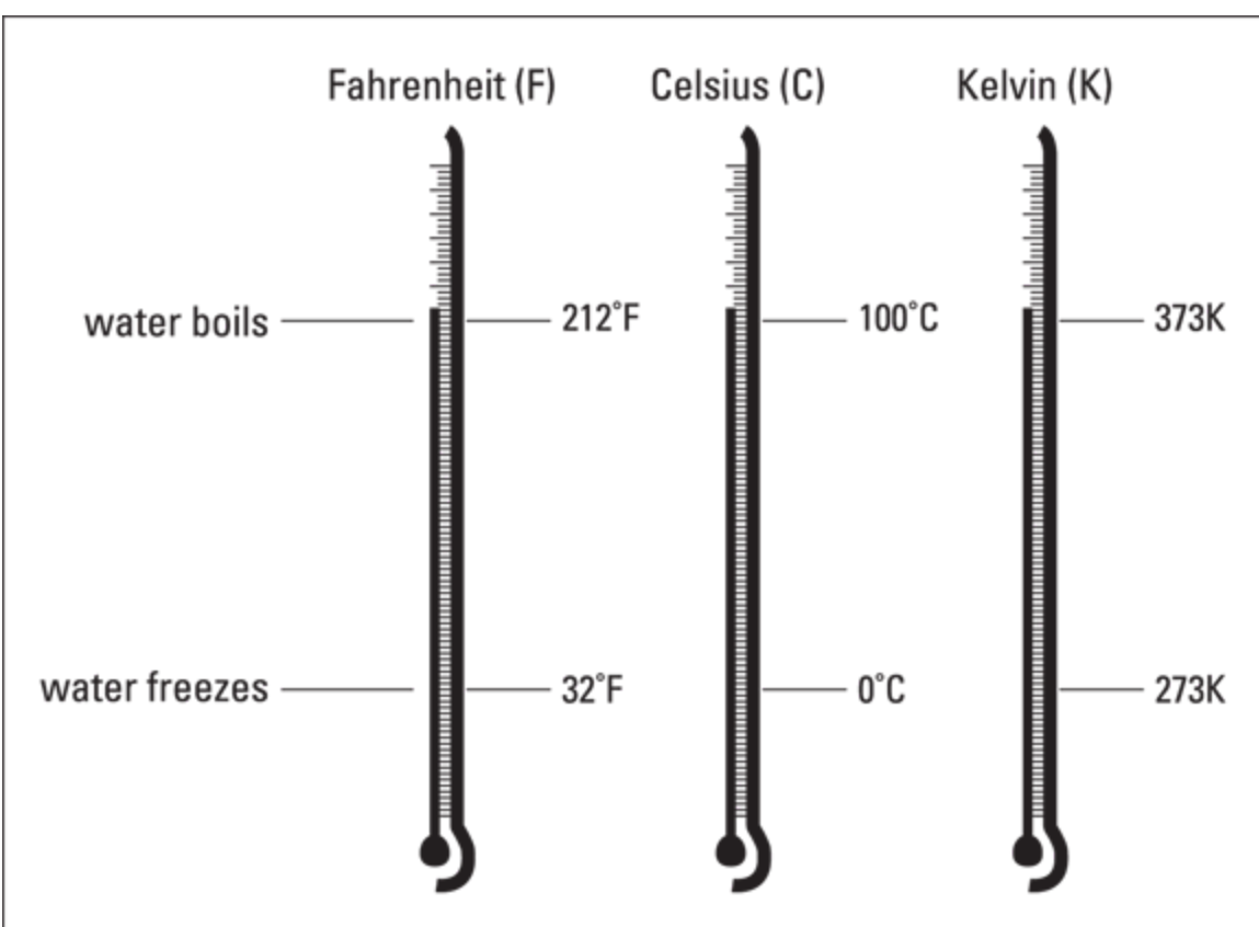
FIGURE 3-4: Comparison of the Fahrenheit, Celsius, and Kelvin temperature scales.
