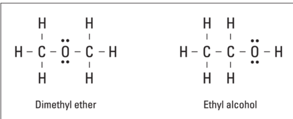
FIGURE 14-5: Two possible compounds of \text{C}_2\text{H}_6\text{O} .
