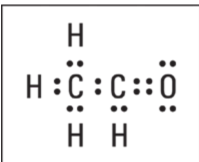
FIGURE 14-8: Electron-dot formula of \text{C}_2\text{H}_4\text{O} .
