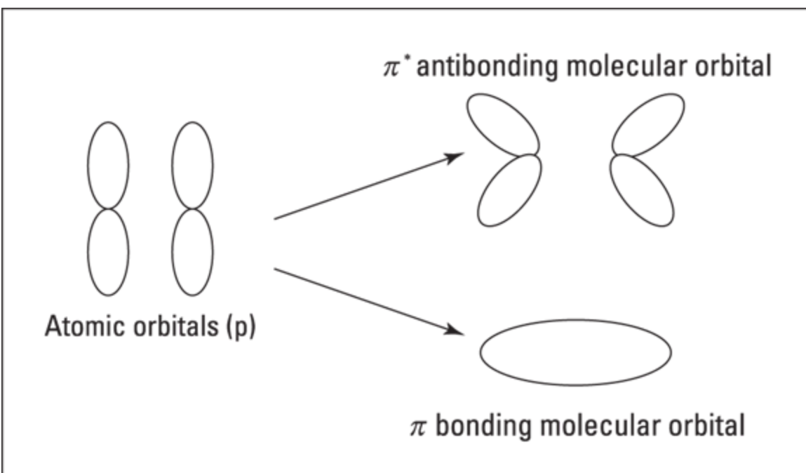
FIGURE 15-9: Formation of pi and pi* molecular orbitals.
