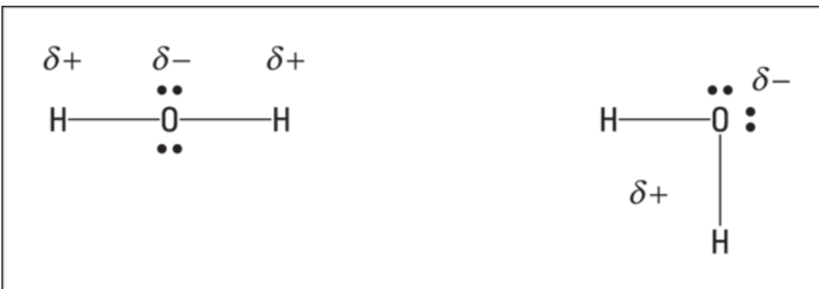
FIGURE 15-3: Two possible Lewis structures of water.
