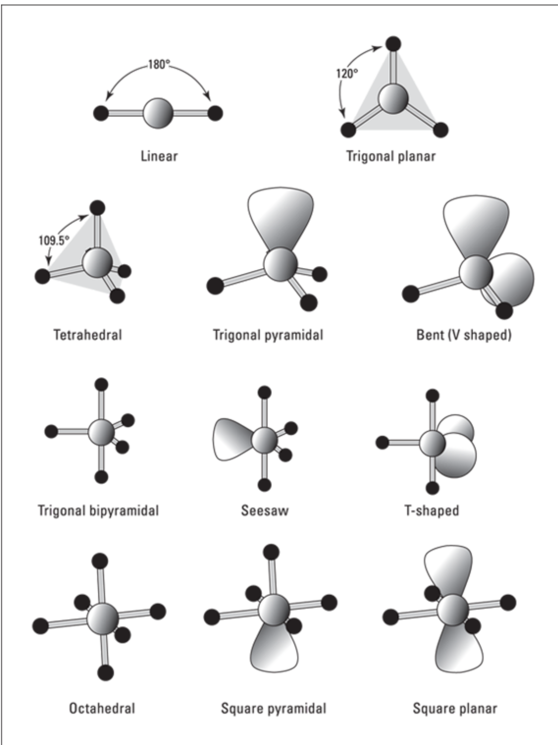
FIGURE 15-4: Common molecular shapes.
